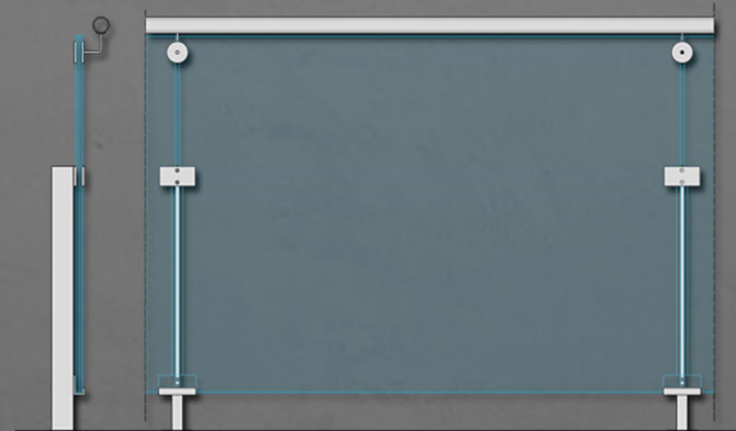
With handrail
